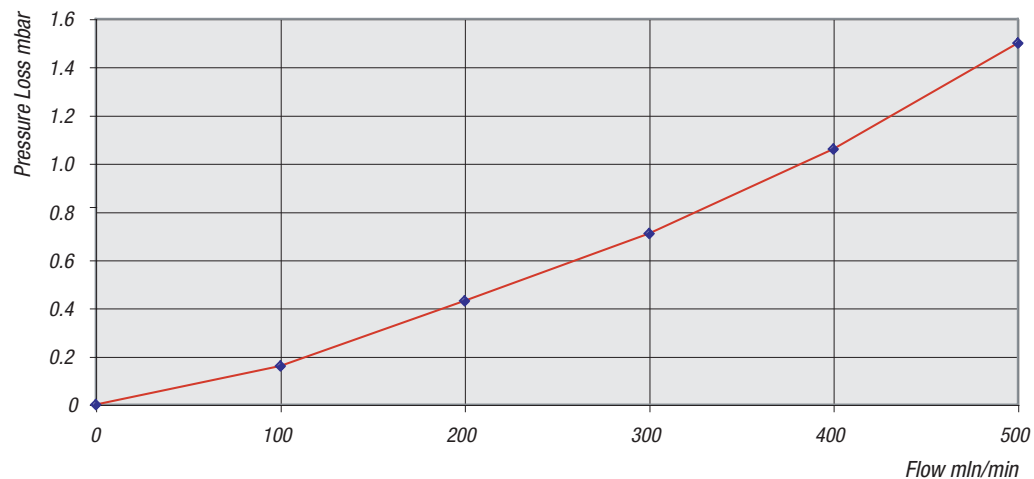
Pressure Loss 500 mln/min (Air)
