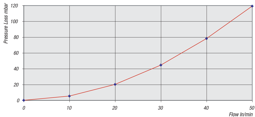
Pressure Loss 50 ln/min (Air)
